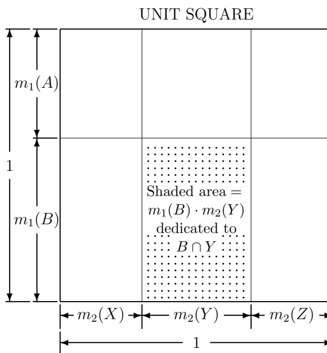
Figure 2-1: Graphical representation of an orthogonal sum
