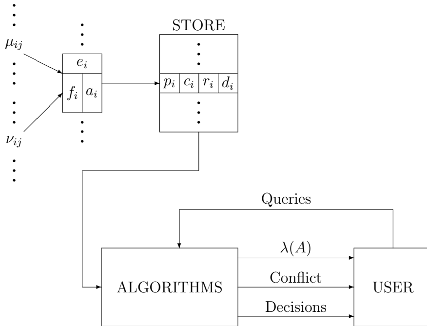
Figure 5–1: Data flow model
